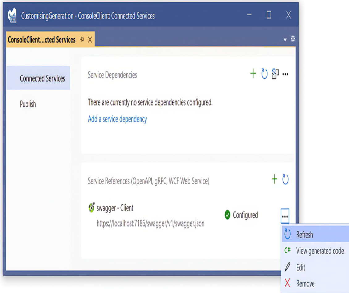
Figure 11.9 Updating the OpenAPI description for an API. Choose Refresh to download the OpenAPI description again and save it to your project. Then NSwag will generate an updated client on the next build.
