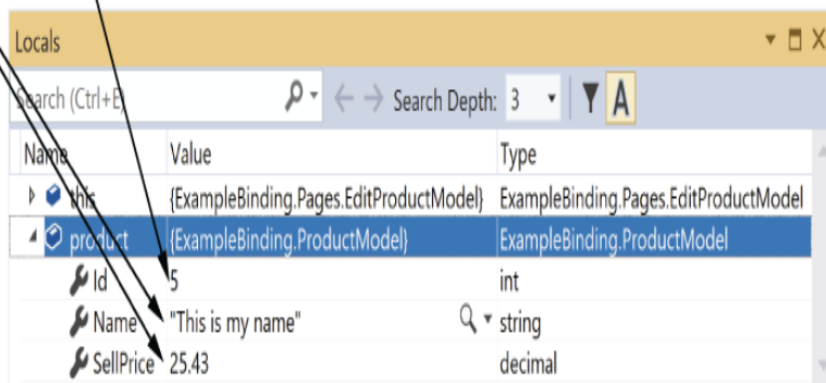
Figure 16.4 Using model binding to create an instance of a model that's used to execute a Razor Page
