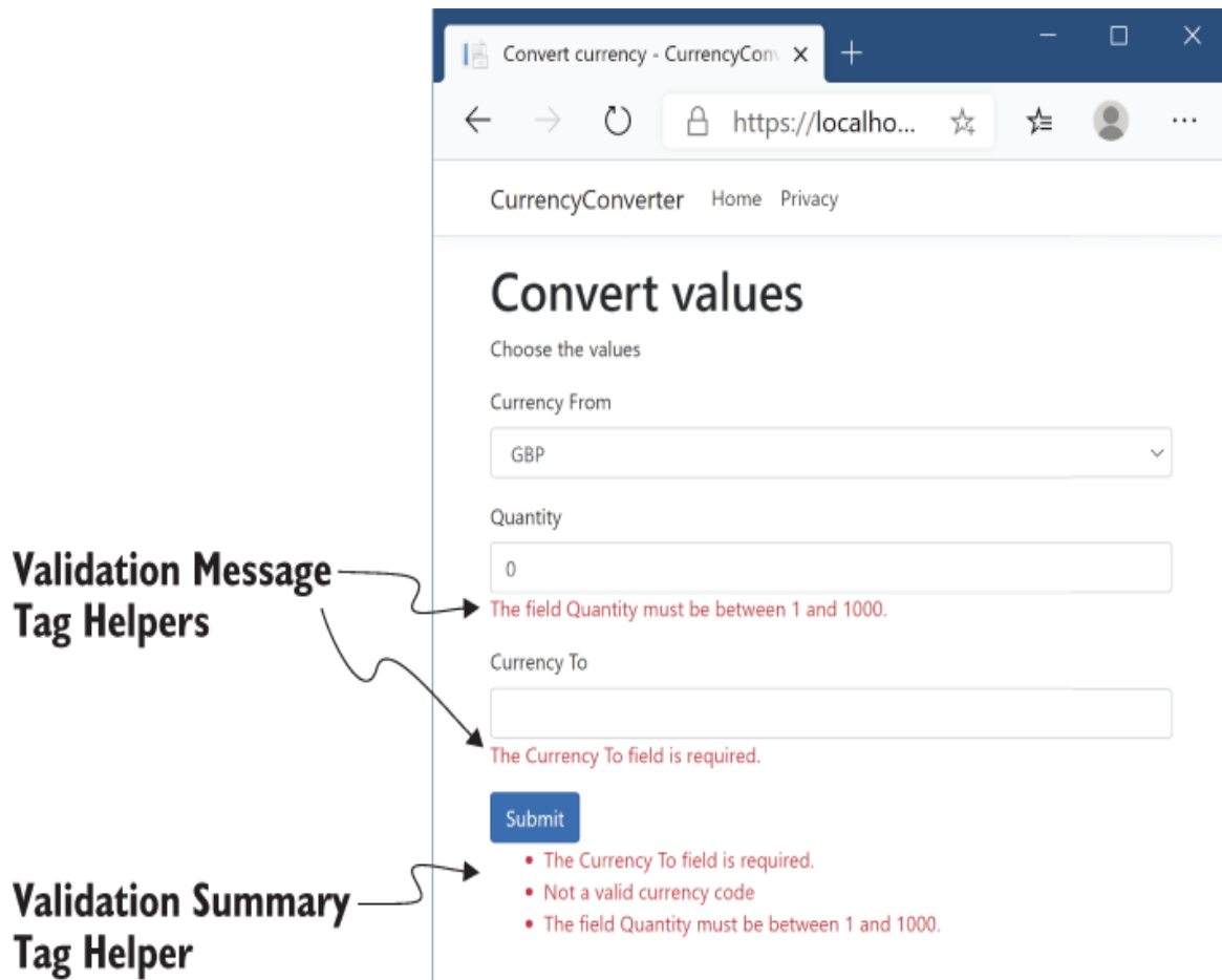
Figure 18.9 Form showing validation errors. The Validation Message Tag Helper is applied to <span> , close to the associated input. The Validation Summary Tag Helper is applied to a <div> , normally at the top or bottom of the form.
