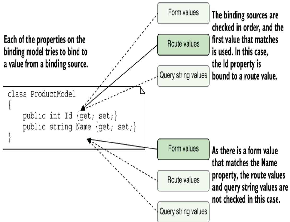
Figure 16.3 Model binding involves mapping values from binding sources, which correspond to different parts of a request.
