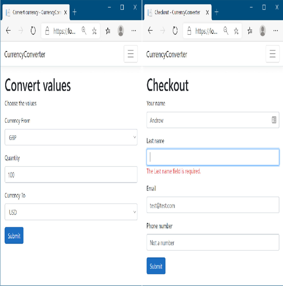
Figure 18.1 The currency converter application forms, built using Tag Helpers. The labels, drop-down lists, input elements, and validation messages are all generated using Tag Helpers.
