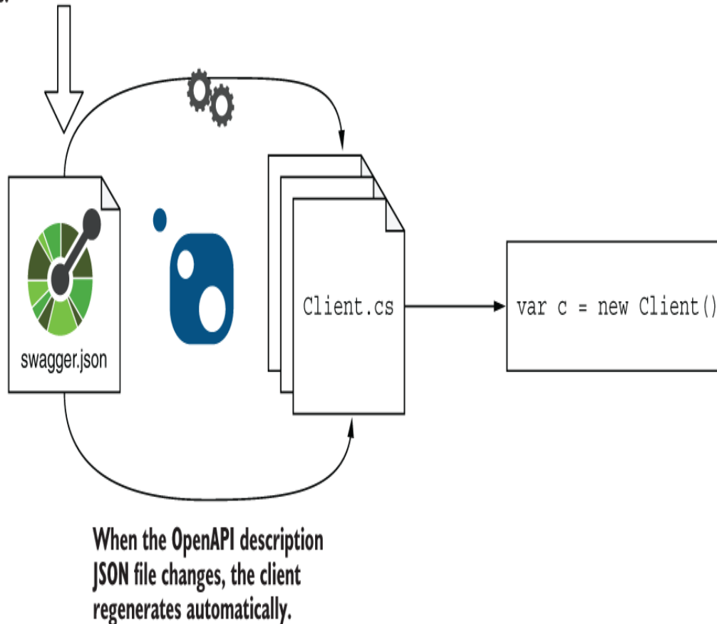
Figure 11.6 Visual Studio or a .NET tool downloads the OpenAPI description locally and installs the code-generation tool from NuGet. When your project builds, the generation tool reads the OpenAPI description and generates a C# class for interacting with the API.
