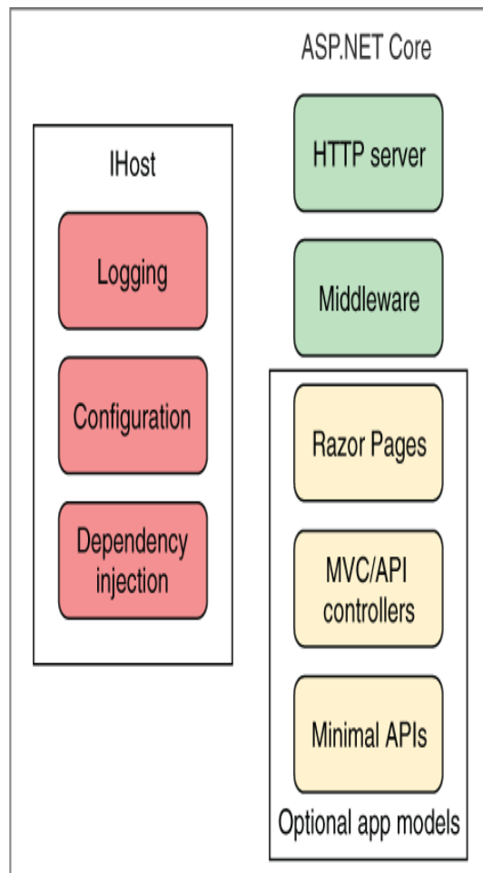
Figure 34.2 ASP.NET Core builds on the generic IHost implementation. IHost provides features such as configuration, DI, and configuration. ASP.NET Core adds HTTP handling on top of that by way of the middleware pipeline, Razor Pages, and API controllers. If you don't need HTTP handling, you can use IHost without the additional ASP.NET Core libraries to create a smaller application.
