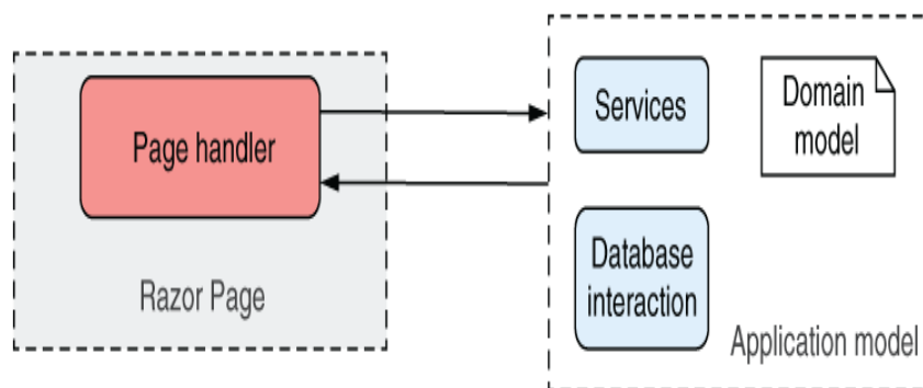
Figure 13.10 When executed, an action invokes the appropriate methods in the application model.
