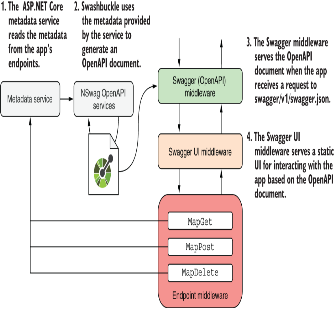
Figure 11.1 Swashbuckle uses ASP.NET Core metadata services to retrieve information about the endpoints in your application and builds an OpenAPI document. The OpenAPI middleware serves this
