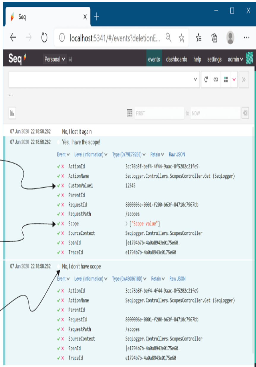
Figure 26.13 Adding properties to logs using scopes. Any scope state that is added using the dictionary approach is added as structured logging properties, but other state is added to the scope property. Adding properties makes it easier to associate related logs with one another.
