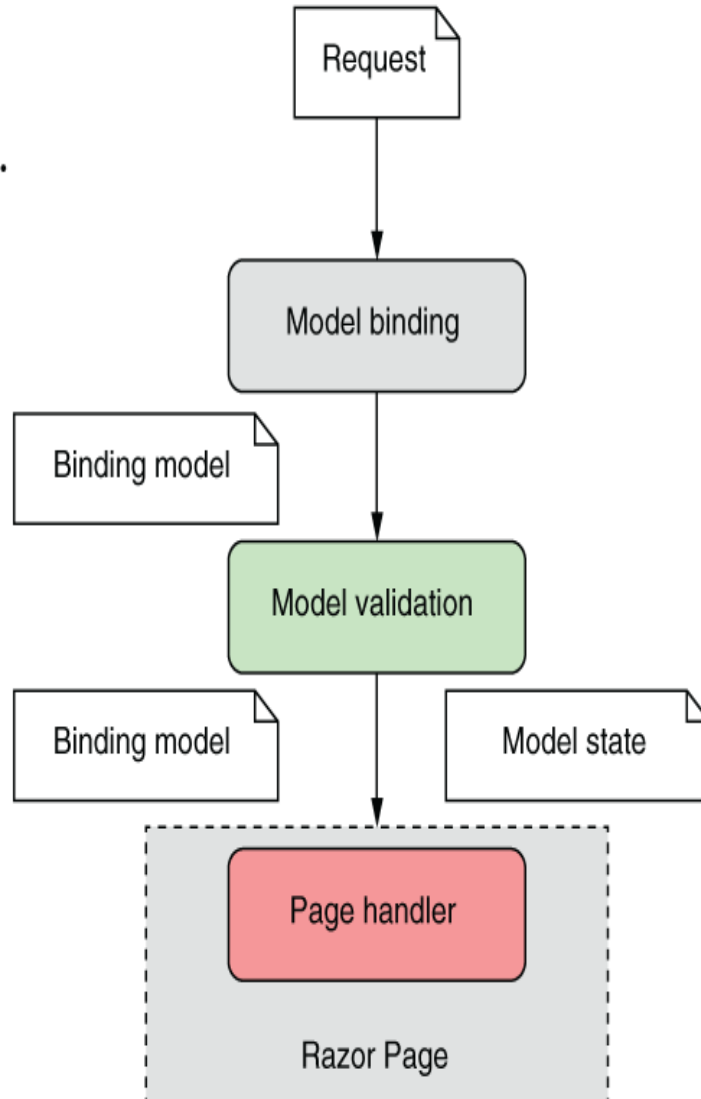
Figure 16.6 Validation occurs after model binding but before the page handler executes. The page handler executes whether or not validation is successful.
