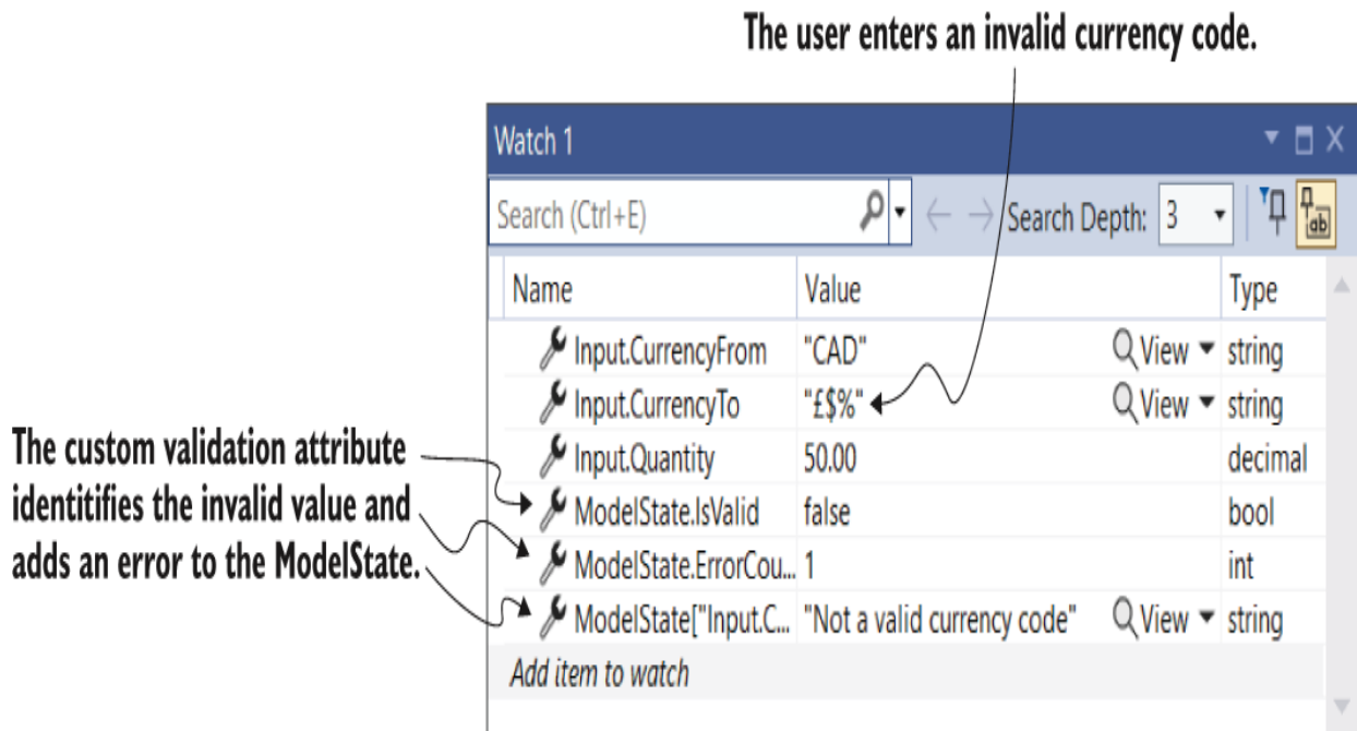
Figure 32.6 The Watch window of Visual Studio showing the result of validation using the custom ValidationAttribute . The user has provided an invalid currencyTo value, £$% . Consequently, ModelState isn't valid and contains a single error with the message "Not a valid currency code".
