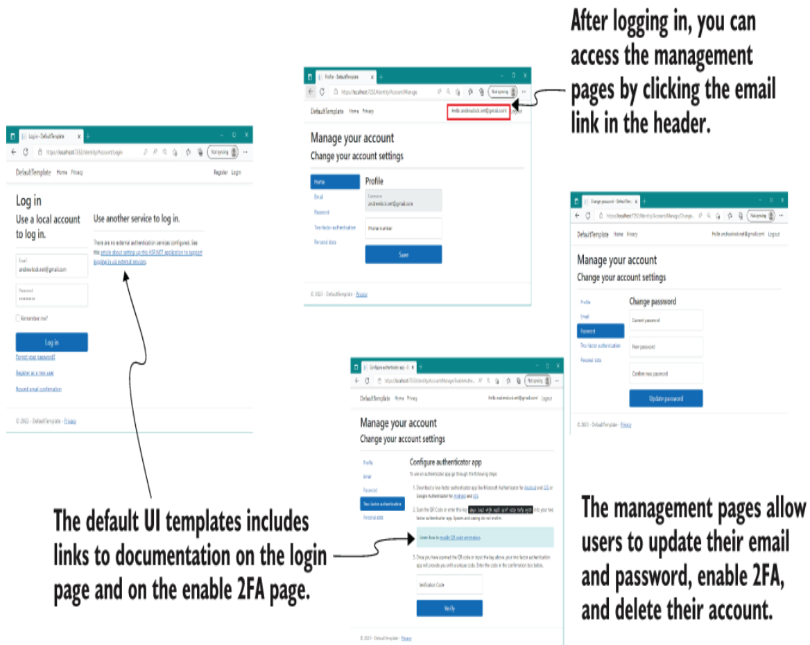
Figure 23.10 Logging in with an existing user and managing the user account. The Login page describes how to configure external login providers, such as Facebook and Google. The user-management pages allow users to change their email and password and to configure MFA.
