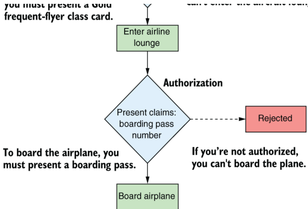
Figure 24.1 When boarding a plane at an airport, you pass through several authorization steps. At each authorization step, you must present a claim in the form of a boarding pass or a frequent-flyer card. If you're not authorized, access is denied.
