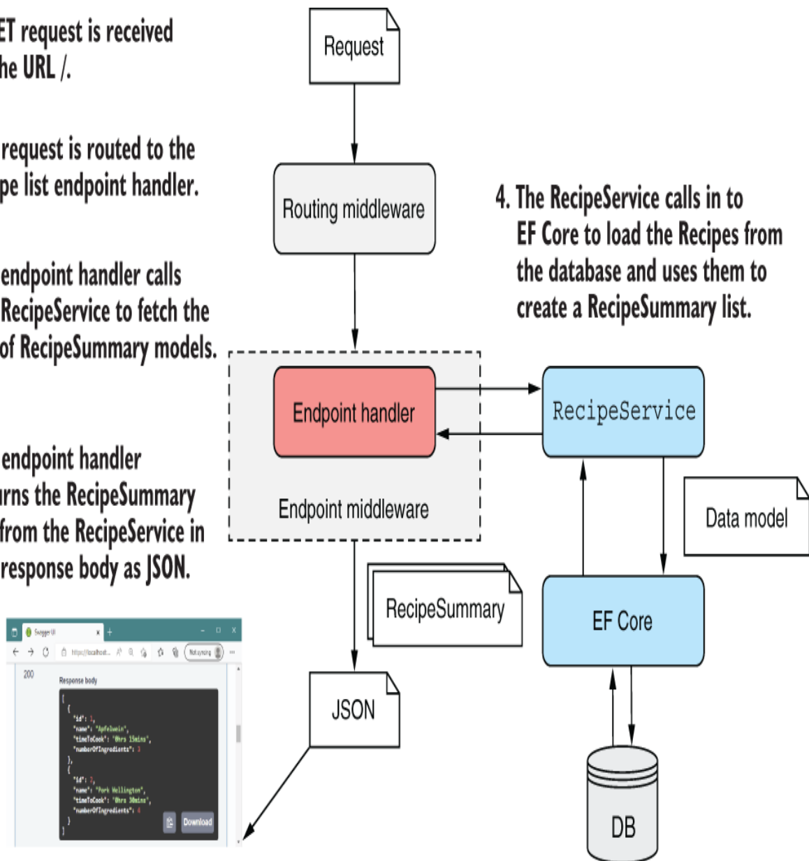
Figure 12.4 Handling a request by loading data from a database using EF Core. Interaction with EF Core is restricted to RecipeService; the endpoint doesn't access EF Core directly.
