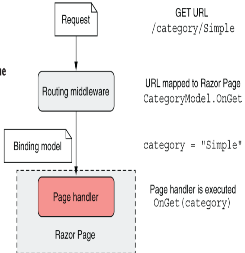
Figure 13.9 Routing a request to a Razor Page and building a binding model. A request to the /category/Simple URL results in the execution of the CategoryModel.OnGet page handler, passing in a populated binding model, category .
