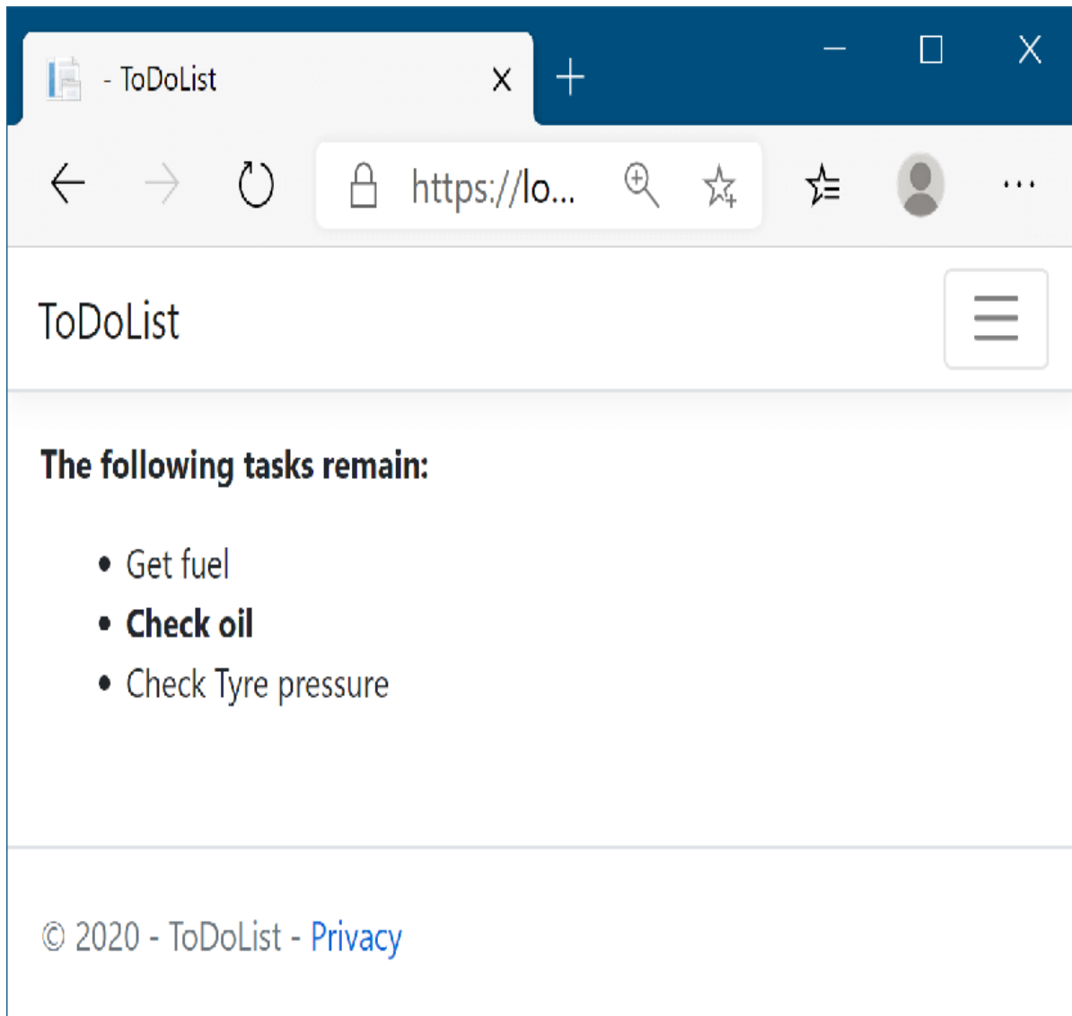
Figure 17.8 The second item, " <strong>Check oil</strong> " has been output using Html.Raw() , so it hasn't been HTML-encoded. The <strong> elements result in the second item being shown in bold
