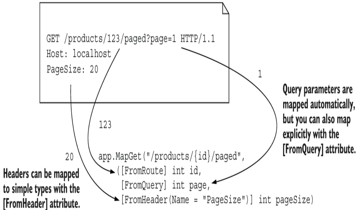
Figure 7.2 Model binding an HTTP get request to an endpoint. The [FromRoute] , [FromQuery] , and [FromHeader] attributes force the endpoint parameters to bind to specific parts of the request. Only the [FromHeader] attribute is required in this case; the route parameter and query string would be inferred automatically.
