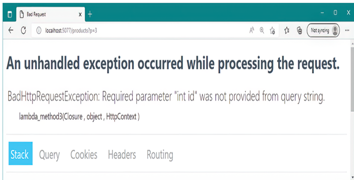
Figure 7.6 If a parameter can't be bound because a value is missing, the EndpointMiddleware throws an exception and returns
