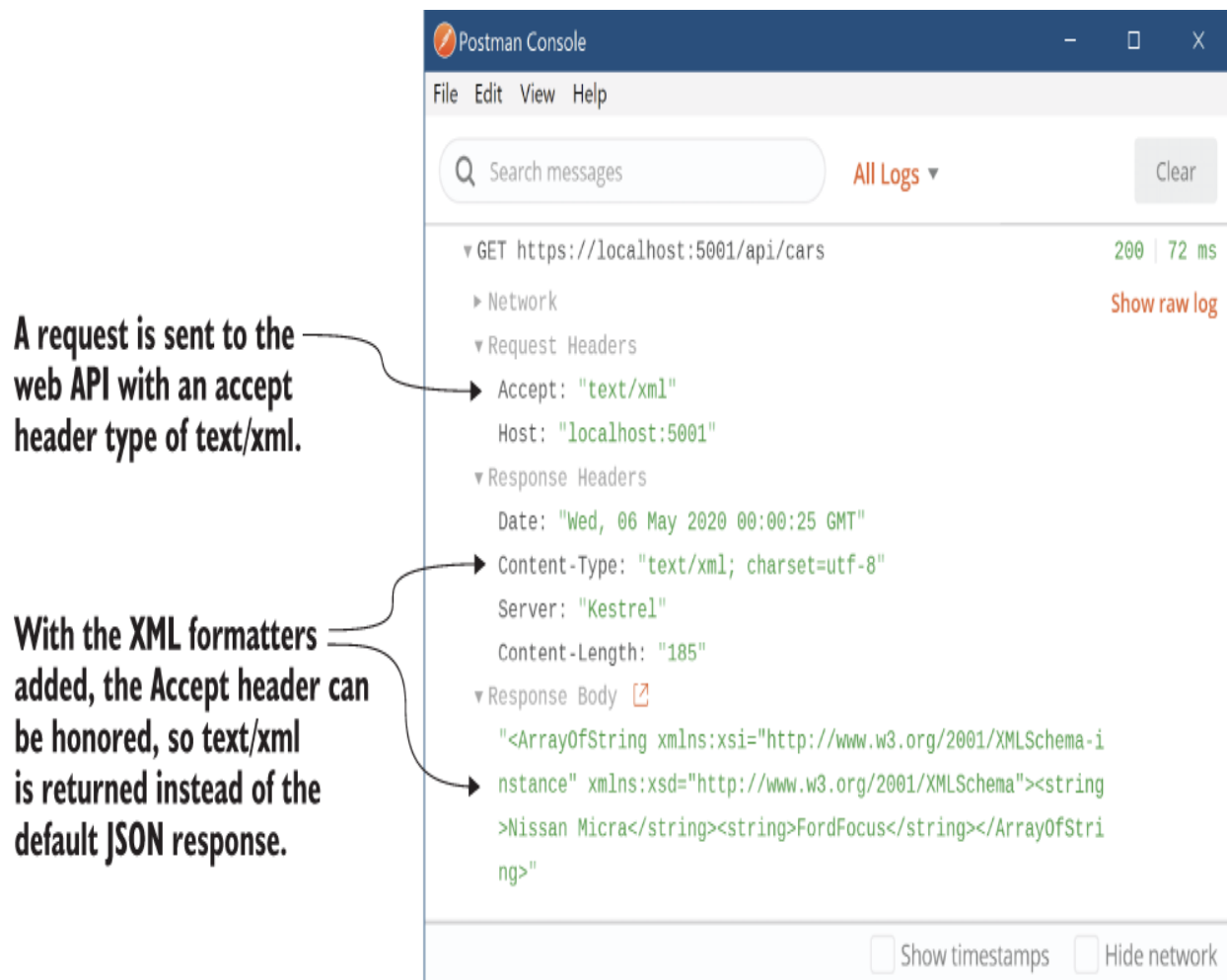
Figure 20.8 With the XML output formatters added, the Accept header's text/xml value is respected, and the response is serialized to XML.
