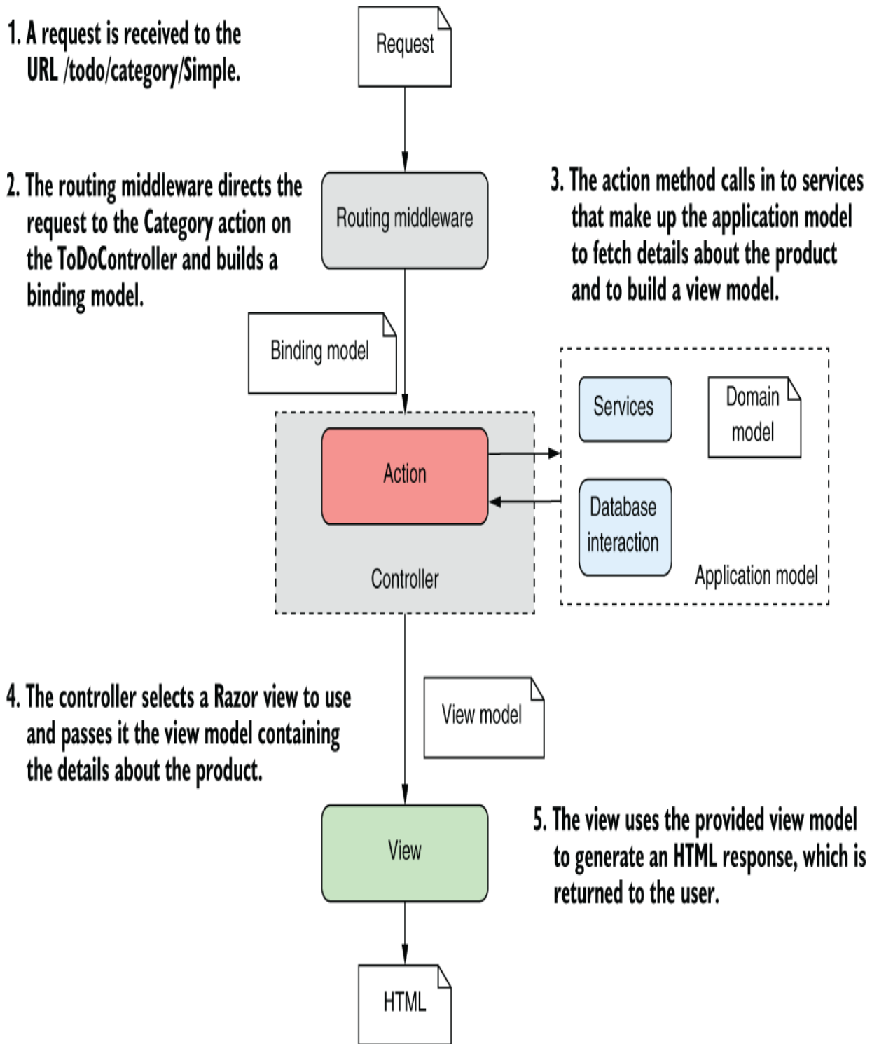
Figure 19.3 A complete MVC controller request for a category. The MVC controller pattern is almost identical to that of Razor Pages, which was shown in figure 13.12. The controller is
