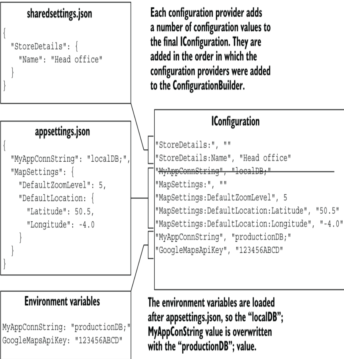
Figure 10.4 The final IConfiguration includes the values from each of the providers. Both appsettings.json and the environment variables include the MyAppConnString key. As the environment variables are added later, that configuration value is used.
