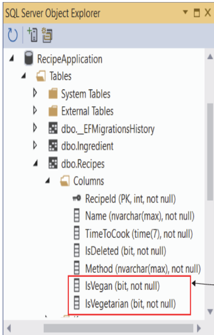
Figure 12.10 Applying the ExtraRecipeFields migration to the database adds the IsVegetarian and IsVegan fields to the Recipes table.
