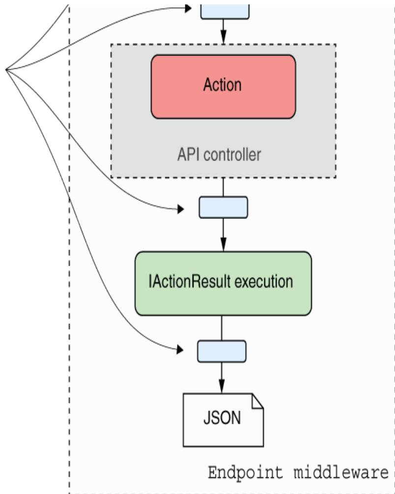
Figure 21.1 Filters run at multiple points in the EndpointMiddleware as part of the normal handling of an MVC request. A similar pipeline exists for Razor Page requests.
