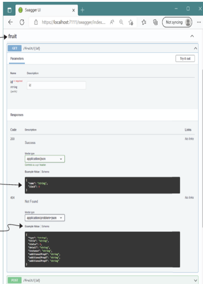
Figure 11.5 Swagger UI groups the endpoints in your application based on the Tag metadata attached to them. The UI uses the metadata added by calling Produces() to document the expected return types and status codes for each endpoint.
