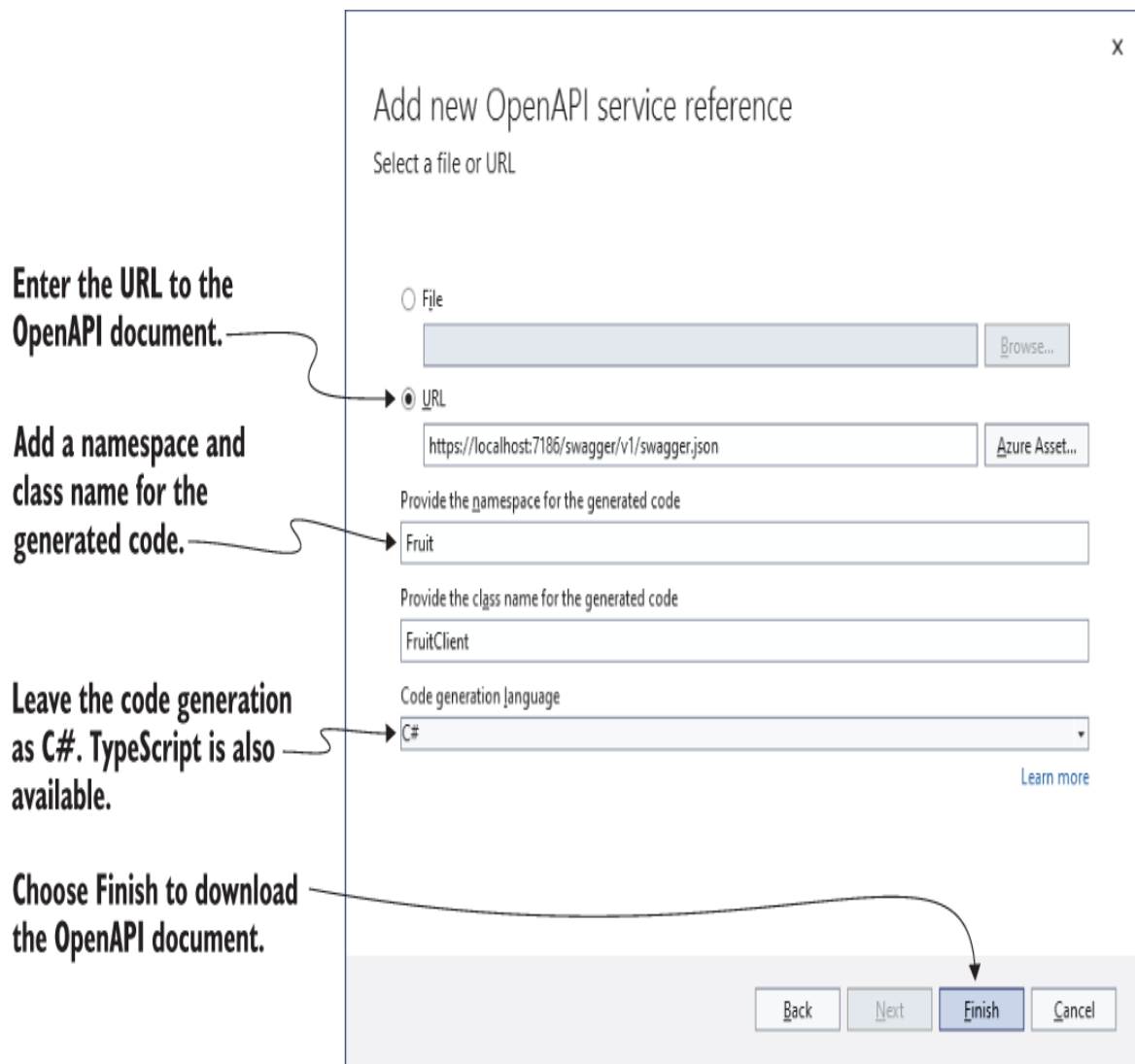
Figure 11.8 Adding an OpenAPI service reference using Visual Studio. Add the link to the OpenAPI document, the code
