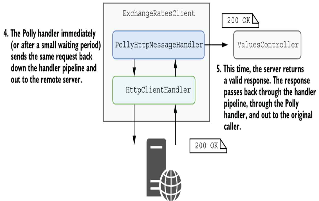
Figure 33.5 Using the PolicyHttpMessageHandler to handle transient errors. If an error occurs when calling the remote API, the Polly handler will automatically retry the request. If the request then succeeds, the result is passed back to the caller. The caller didn't have to handle the error, making it simpler to use the HttpClient while remaining resilient to transient errors.
