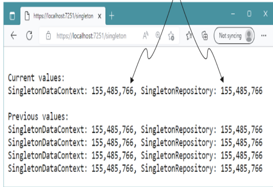
Figure 9.9 Any service registered as a singleton always returns the same instance. Consequently, all the calls to the RowCounts handler return the same value, both within a request and between requests.
