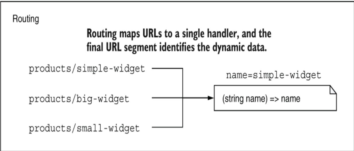
Figure 6.2 If you use static URL-based mapping, you need a different handler for every product in your product range. With a query string, you can use a single handler, and the query string contains the data. With routing, multiple URLs map to a single handler, and a dynamic parameter captures the difference in the URL.
