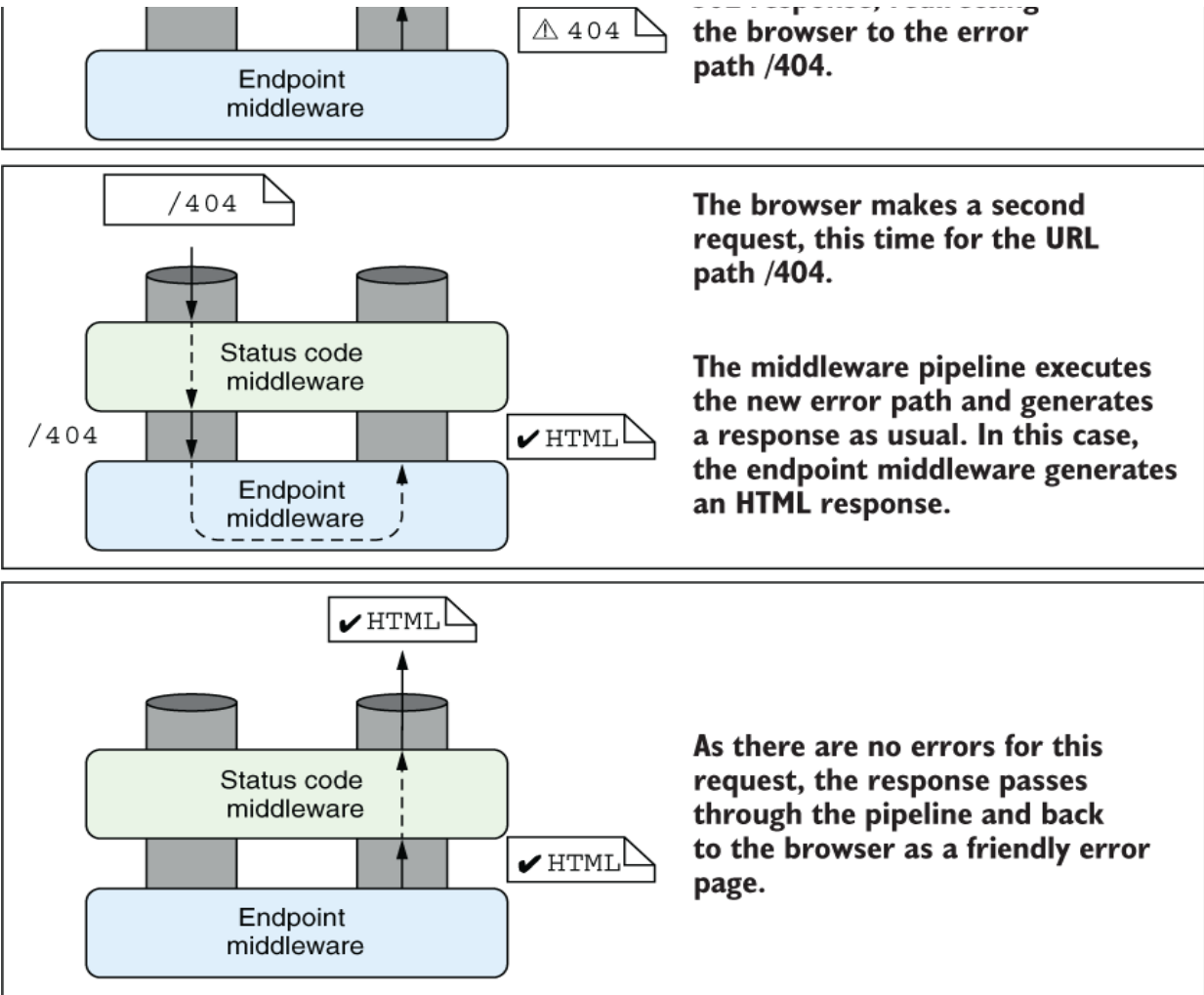
Figure 15.8 StatusPagesMiddleware returning redirects to generate error pages. A request to the / path returns a 404 response, which is intercepted by the status code middleware and converted to a 302 response. The browser makes a second request using the /404 path to generate the HTML response.
