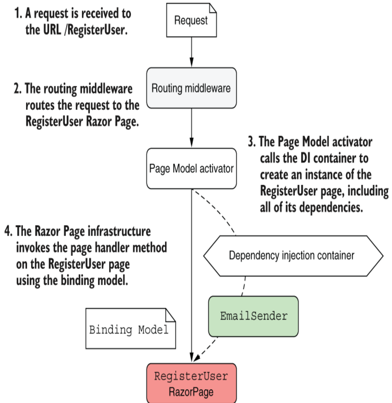
Figure 8.5 The ASP.NET Core hosting model uses the DI container to fulfill dependencies when creating Razor Pages.
