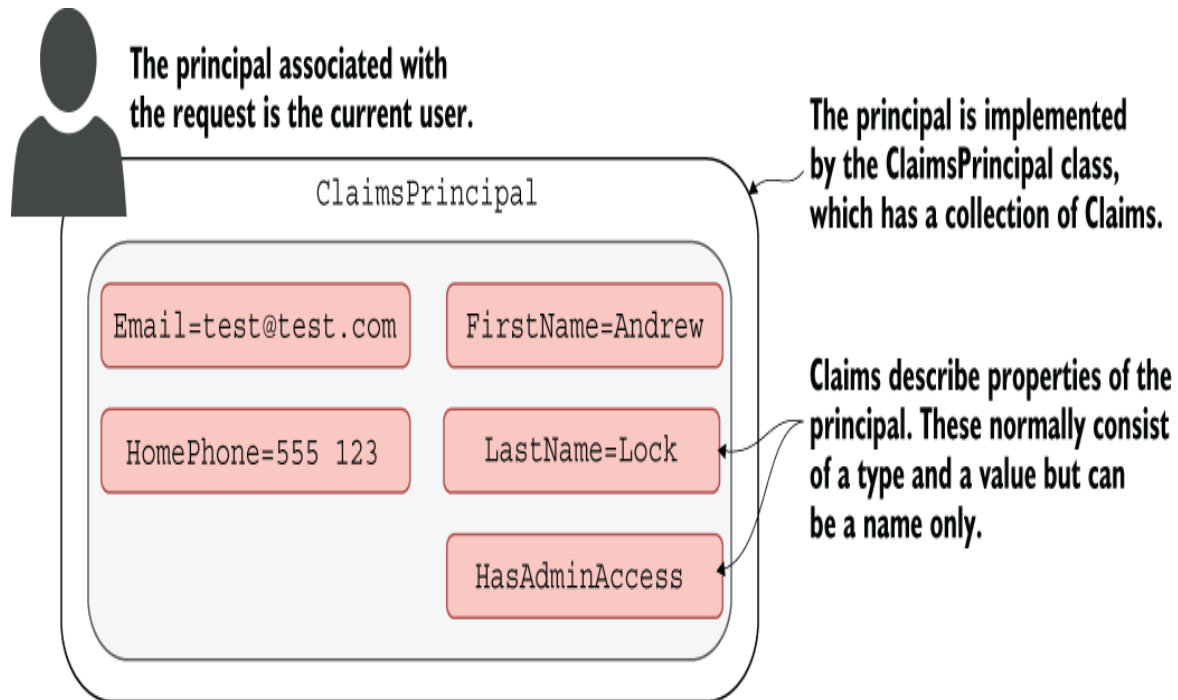
Figure 23.1 The principal is the current user, implemented as ClaimsPrincipal . It contains a collection of Claims that describe the user.
