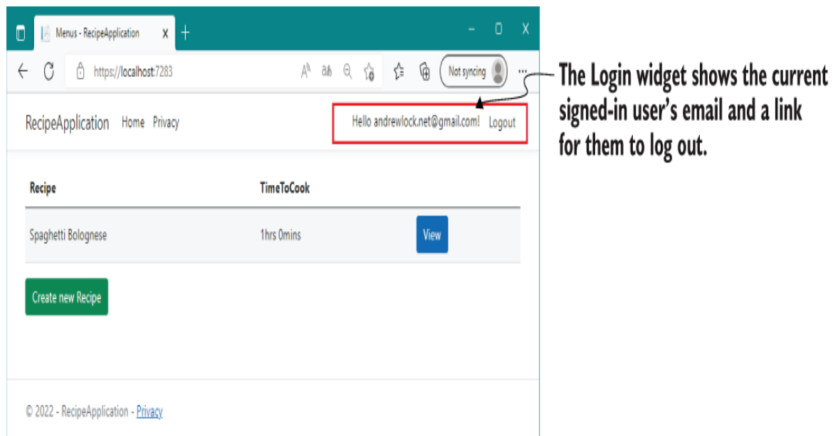
Figure 23.11 The recipe app after adding authentication, showing the Login widget
