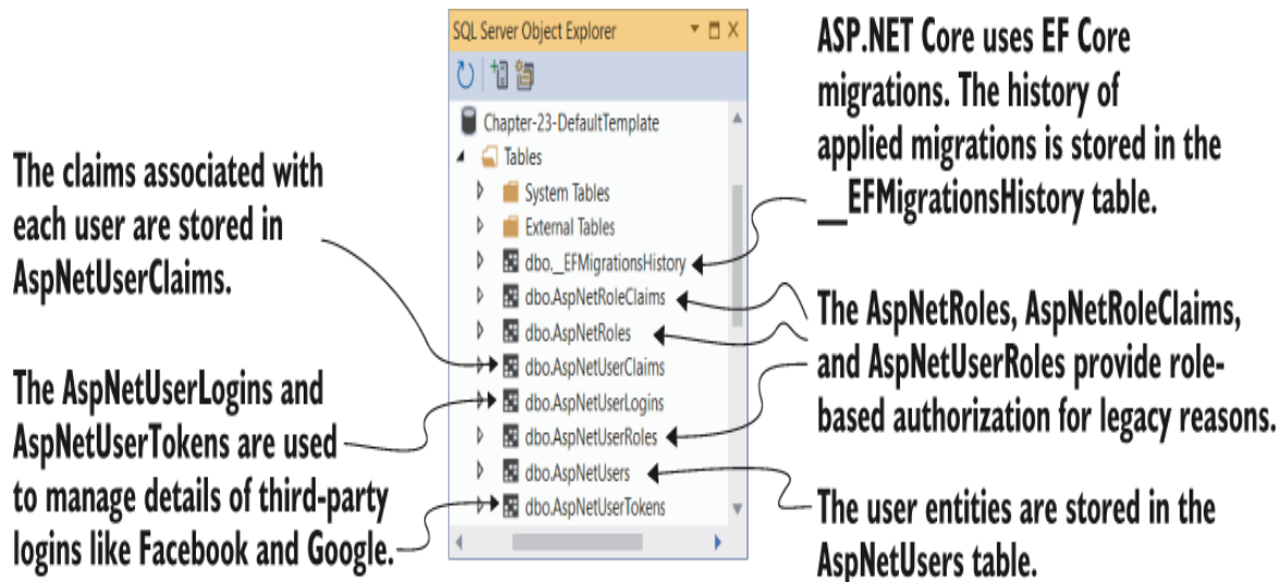
Figure 23.7 The database schema used by ASP.NET Core Identity
